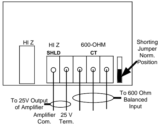
FIGURE 3: Match 25V Speaker Line to 600/500 Ohm Input
