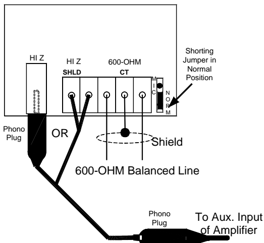
FIGURE 1: Input Matching Transformer
