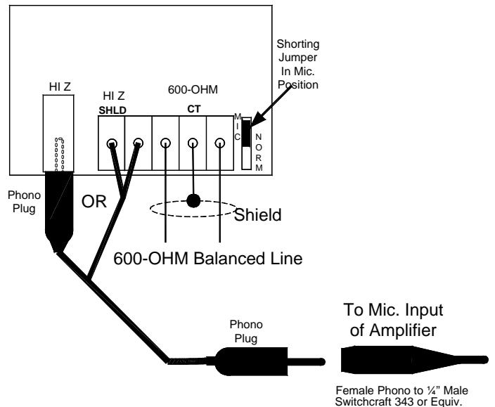
FIGURE 2: Connection to Microphone Input
