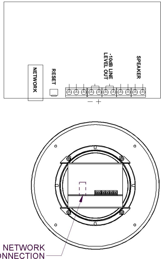
Figure 1. VIP-120A-SA Connections
